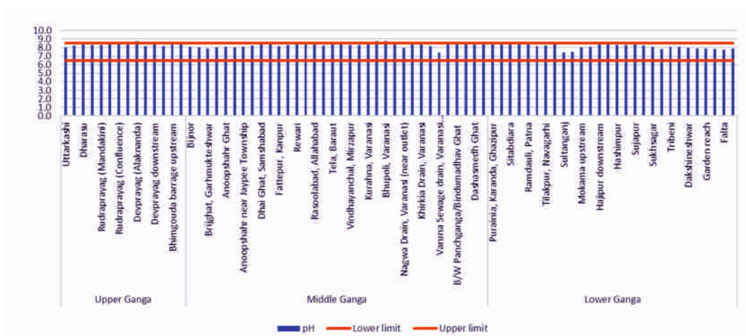
Figure 4.1 pH level in the upper, middle and lower stretches of the Ganga River
