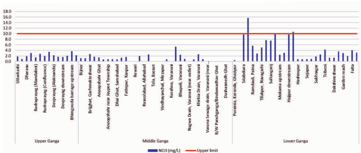
Figure 4.3 Nitrate concentration in the upper, middle and lower stretches of the Ganga River
