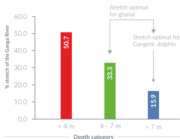
Figure 2.1 Percent suitability of the Ganga River for priority aquatic species in terms of water depth
